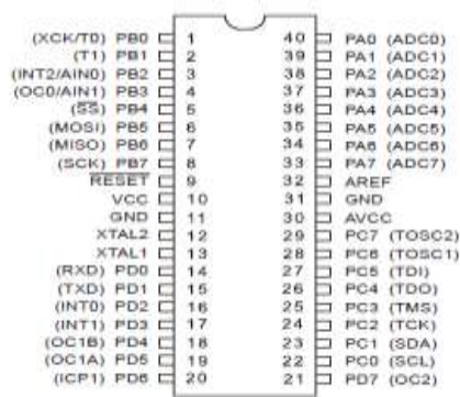
Fig. PIN diagram of ATmega16
