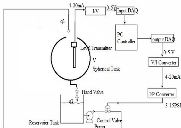
Figure 1: Block Diagram of Process
