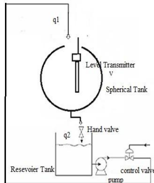
Figure:2 Valve Connection Diagram
