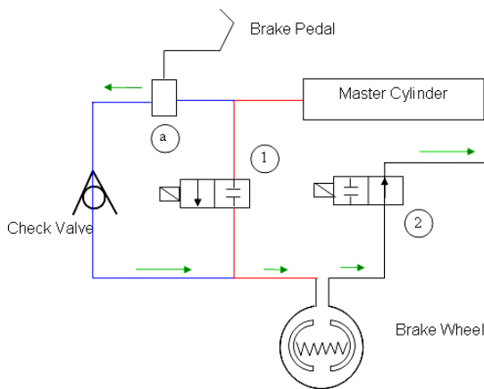
Fig. 1 Schematic Circuit of Badls Fig. 2 Working of the Badls Circuit
