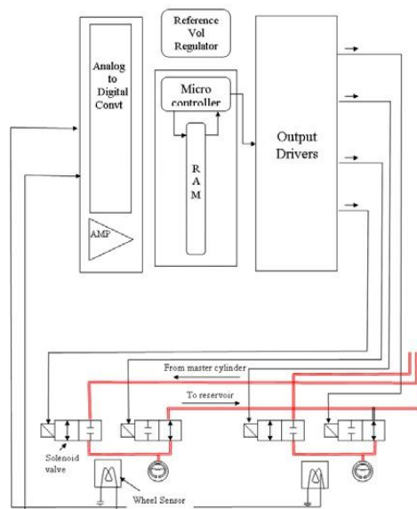
Fig. 3 Proposed Architecture of System
