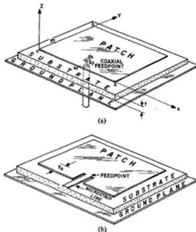
Fig. 1 The structure of microstrip antenna.
