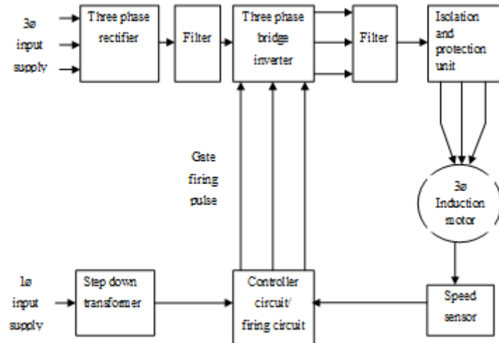
Fig 2: Block diagram of driving circuit
