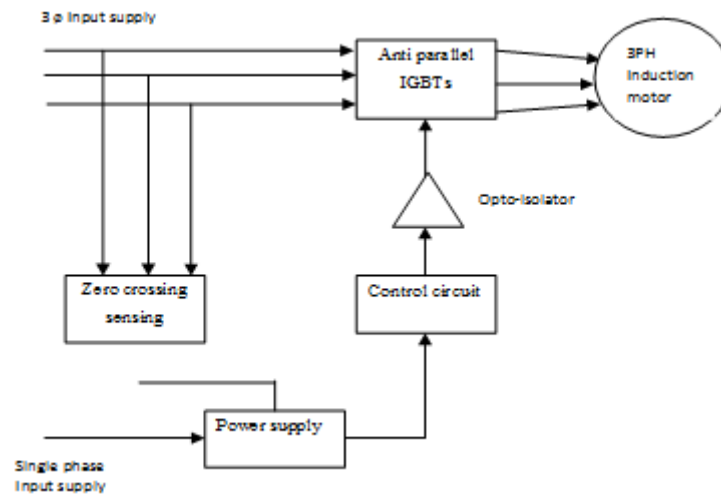
Fig 3: Block diagram of soft starter circuit
