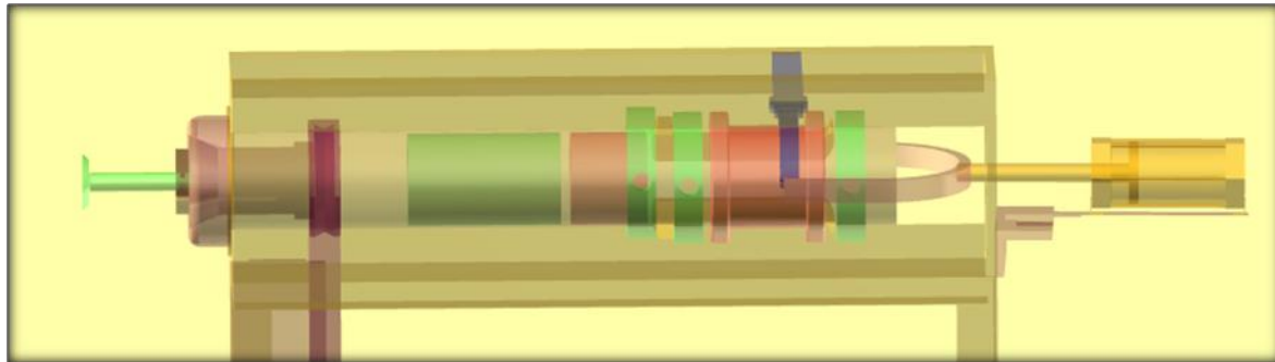
Fig 1: - Arrangement of tappet face polished machine
