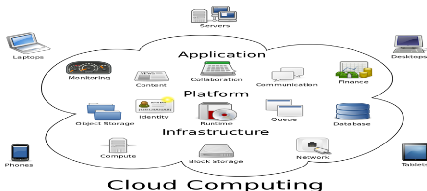
Fig1. Cloud Computing
