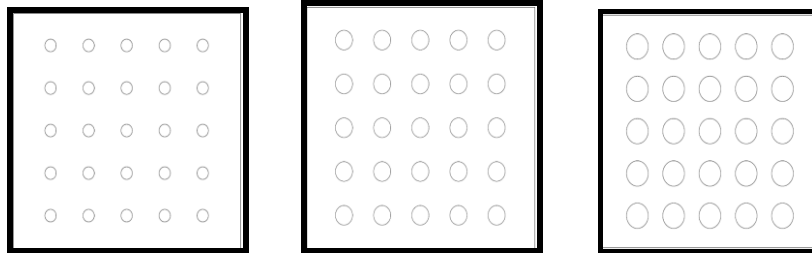
Fig.No.1:- Proposed dimpled plates with variation in diameter of dimples (In-line arrangement)
