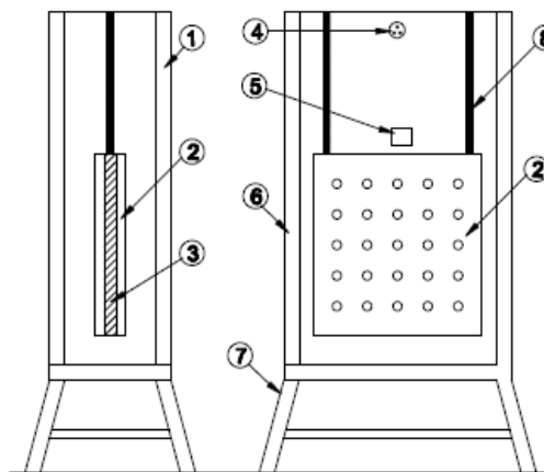
Fig.No.3 :- Schematic diagram of natural convection apparatus
