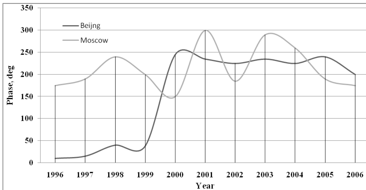
Figure 2 – Phases (degree) for the annual average diurnal variation for Moscow and Beijing neutron monitors
