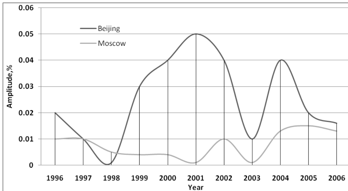
Fig.1- Amplitudes (%) for the annual average diurnal variation for Moscow and Beijing neutron monitors.
