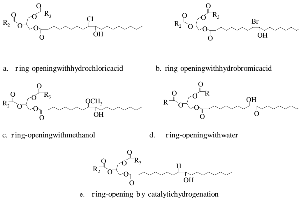
Figure 1.1.6 Polyols from ESO (ring opening with different chemical agents)
