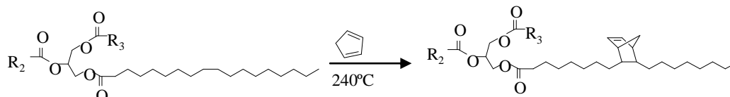
Figure 1.1.13 Diels-Alder reaction
