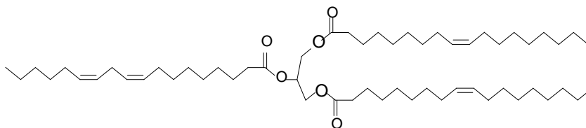
Figure 1.2 Triglyceride molecule.
