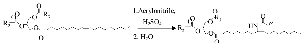
Figure 1.1.11 Ritters Reaction
