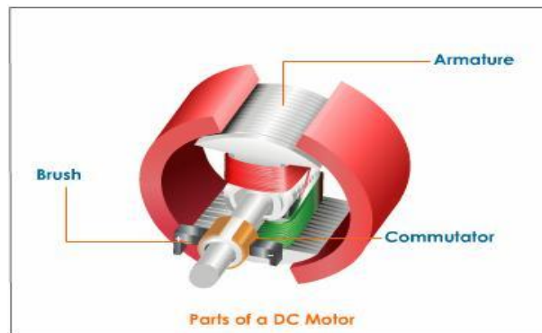
Fig. 1. Parts of a DC motor ]
