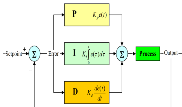
Fig. 2. Schematic of the PID Controller
