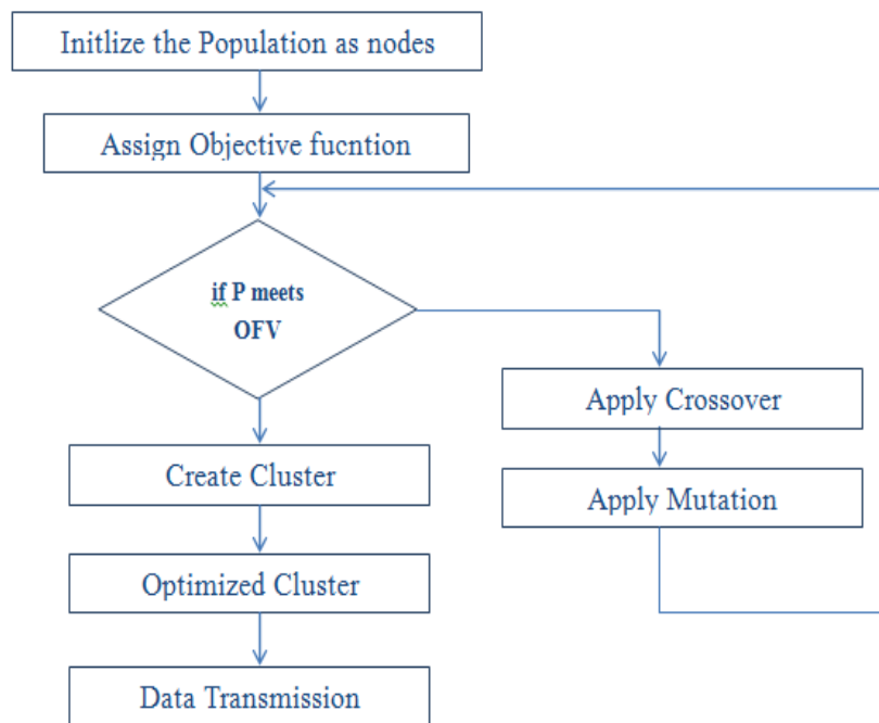
Figure 3.2 GA Flowchart used for WSN [19]
