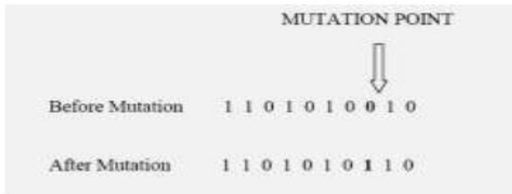
Figure 3.4 Mutation [20]
