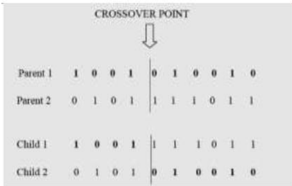
Figure 3.3 Crossover [20]
