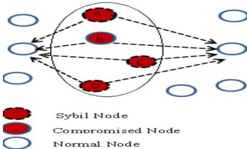
Figure 1.3 Sybil Node [17]
