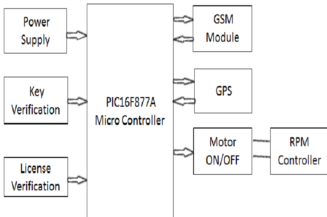
Fig. 2: System Architecture.
