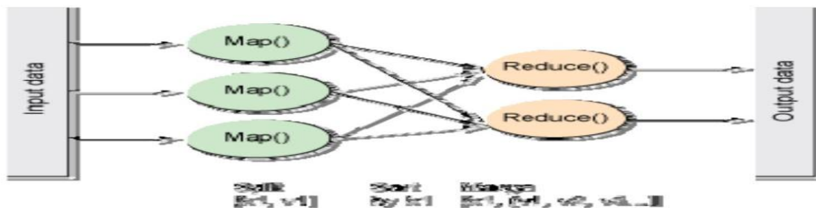
Fig 3: Map reduce
