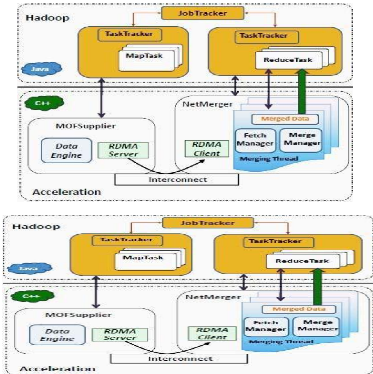
Fig 2: Hadoop structure
