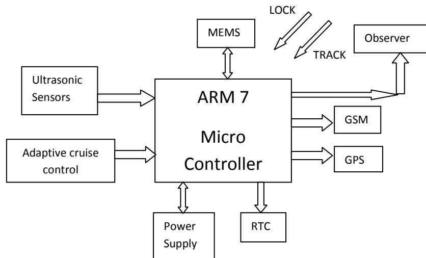
Fig.2 The block diagram of the system [2]
