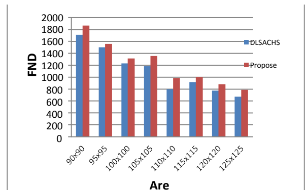
Fig: 6 Value of FND when area is increased
