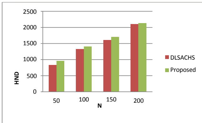
Fig :7 Value of HND when number of nodes is increased
