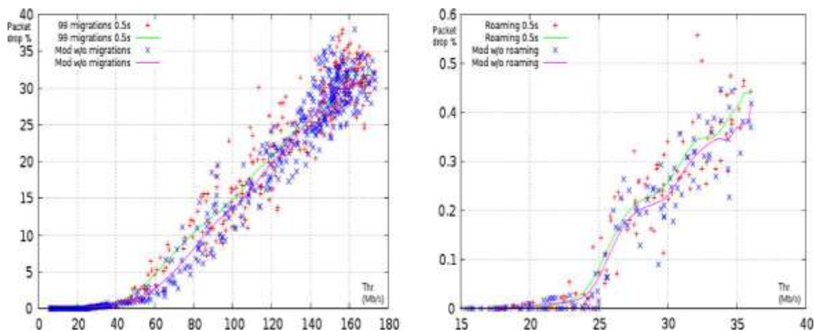
a. Patched Snort: w/o roaming vs roaming
