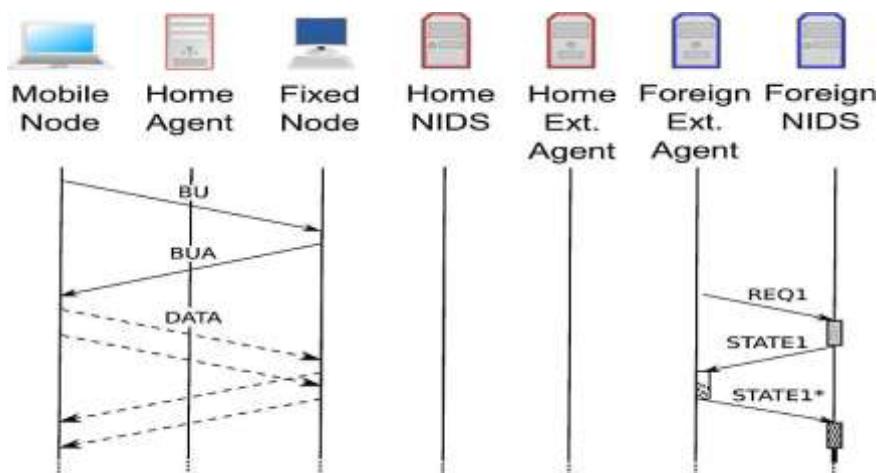
Fig-3 Route optimization sequence diagram
