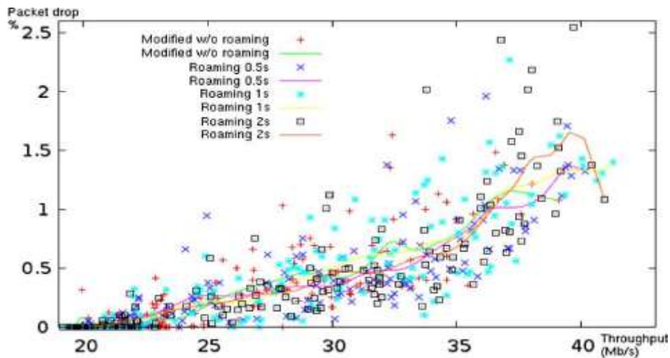
Fig-5 Patched Snort performance with and without roaming for both traces
