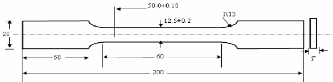
Fig.2 Standard Specimen sizes
