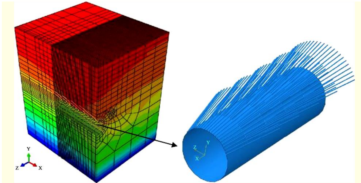
Figure 4. Numerical analysis of the tunnel maintenance method model using the umbrella arch strategy [6] .
