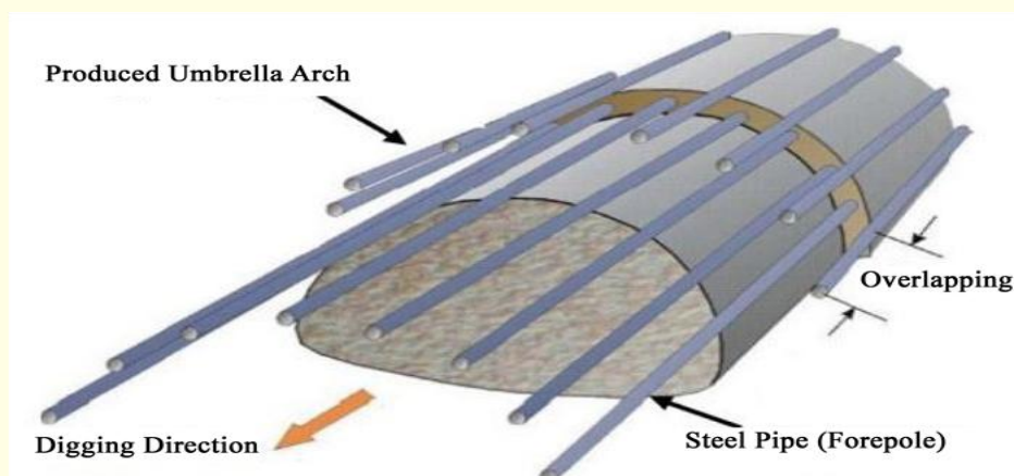
Figure 1. Overview of umbrella arch method [5].
