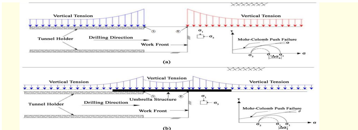
Figure 2. Vertical stress distribution along the longitudinal axis of the tunnel crown and stress on top of the drilling profile. (a) Not using the umbrella method; (b) Using the umbrella method.
