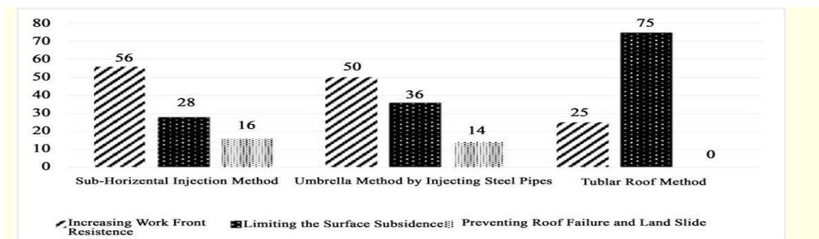
Figure 3. The effects of each of umbrella methods by separating the objects of the method [1].
