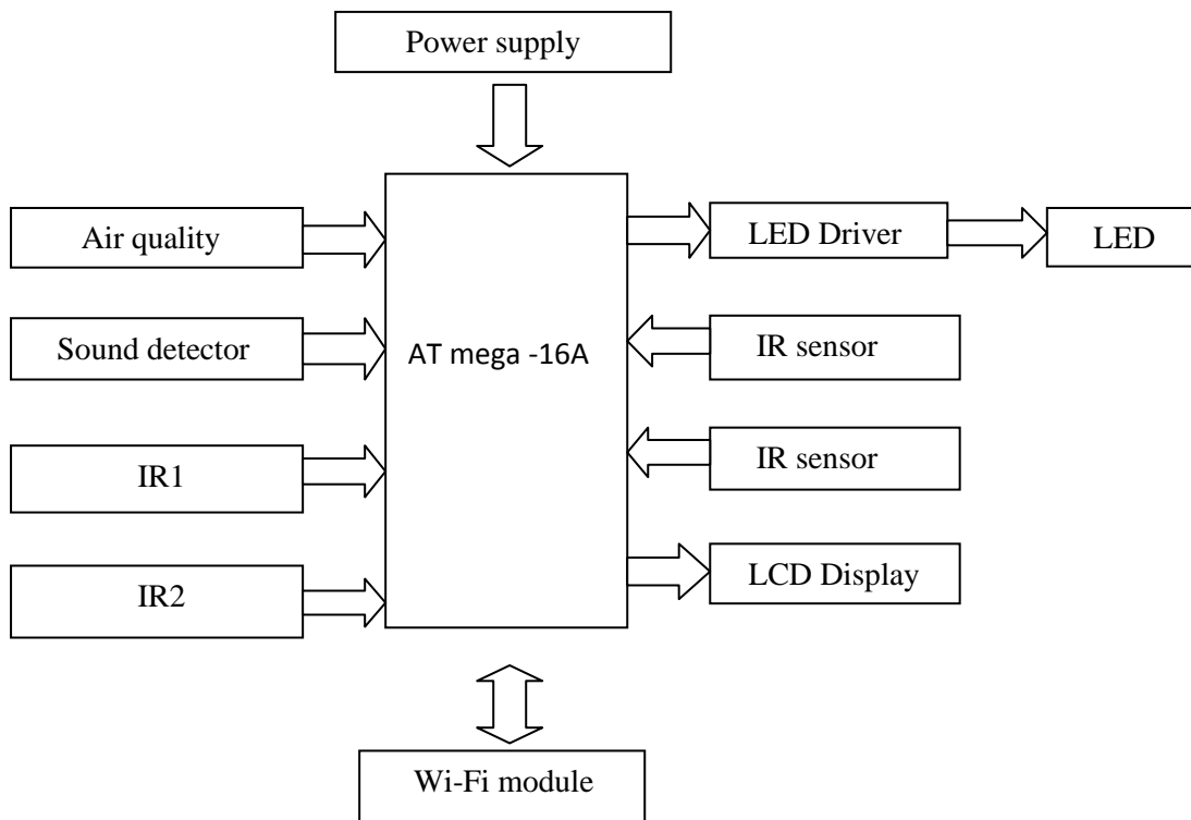
Fig : Block diagram of IOT based Smart City
