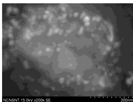
Figure 4. SEM image of green synthesized \text{Fe}_3\text{O}_4 nanoparticles
