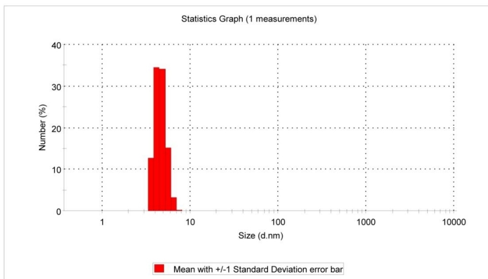
Figure 6. Size distribution of green synthesized \text{Fe}_3\text{O}_4 nanoparticles
