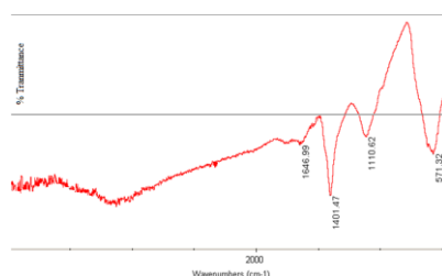
Figure 3. FTIR spectrum of green synthesized \text{Fe}_3\text{O}_4 nanoparticles
