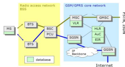
Fig2. GSM/GPRS network architecture
