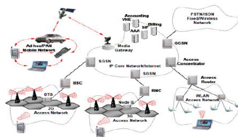
Fig5.Architecture of 4G network [4]
