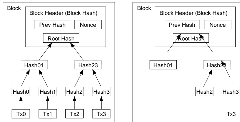
Transactions Hashed in a Merkle Tree Block
