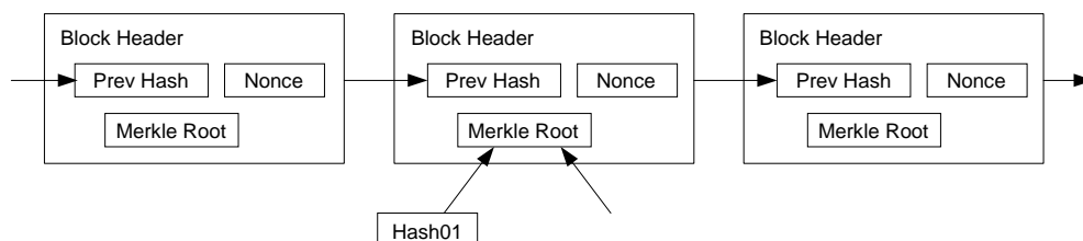
Longest Proof-of-Work Chain
