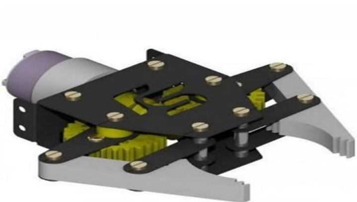
Fig.2 Gripper diagram
