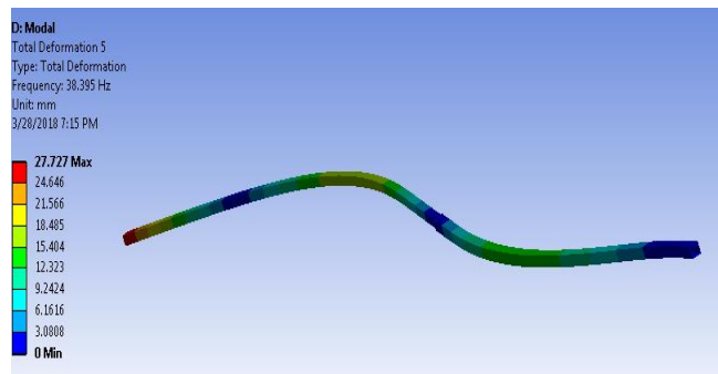
Fig.6 Frequency of deformation.
