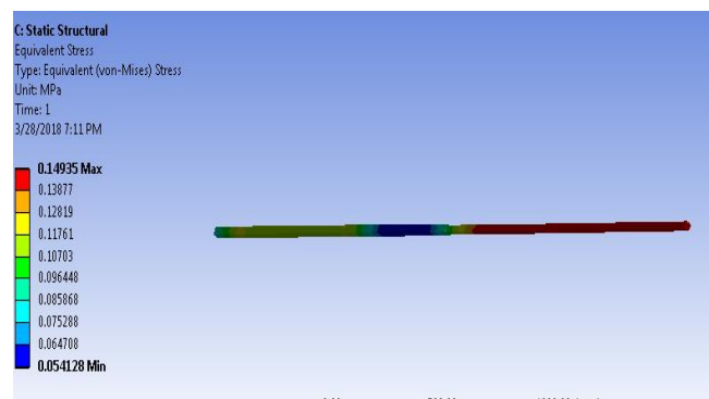
Fig.5 Equivalent stress.
