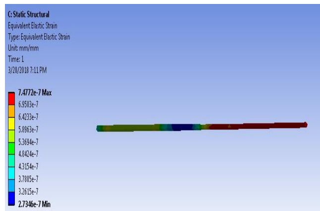
Fig:8 Elastic tension.
