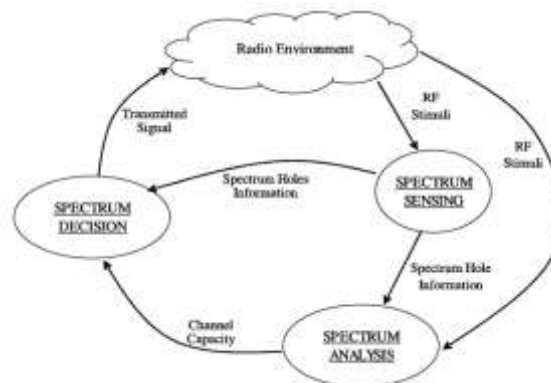
Figure 1. Cognitive cycle
