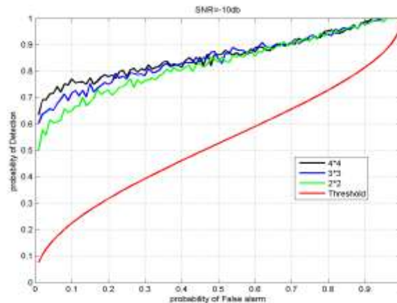
Figure 4. MIMO based P_d SNR=-10 db.
