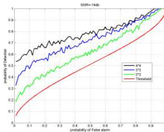
Figure 3. MIMO based P_d SNR=-14 db.
