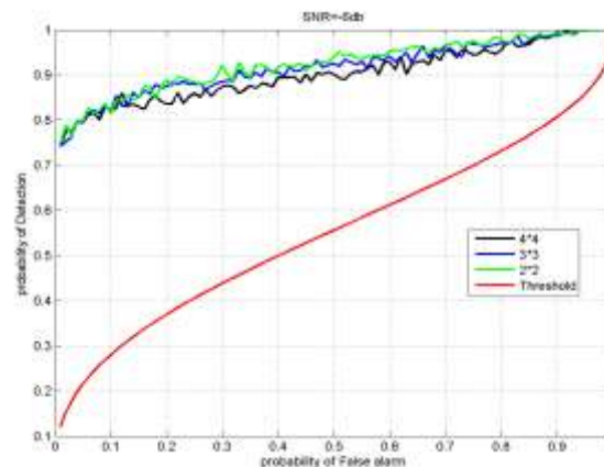
Figure 5. MIMO based P_d SNR=-6 db.
