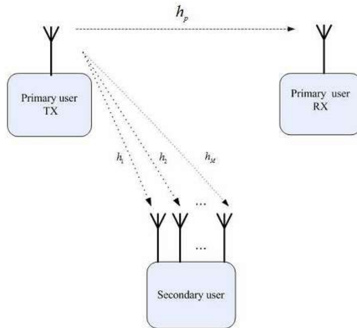
Fig. 2. MIMO for Spectrum Sensing.
