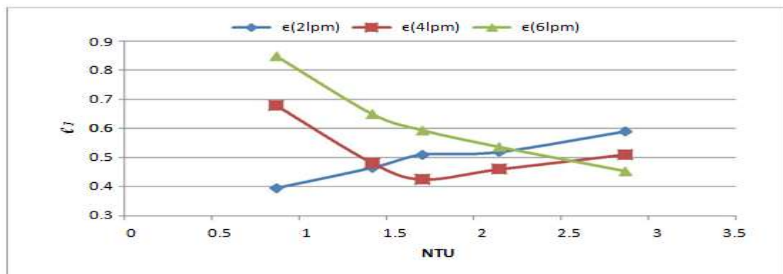
Fig 8 shows the variation of effectiveness with number of transfer unit in bphe for parallel and counter flow .it
