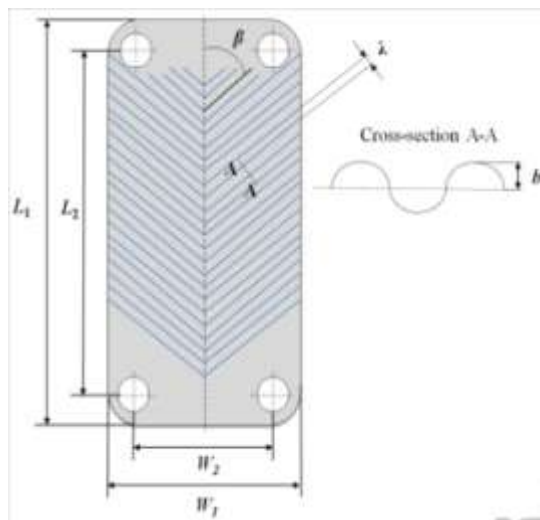
Fig 1 corrugated plate
