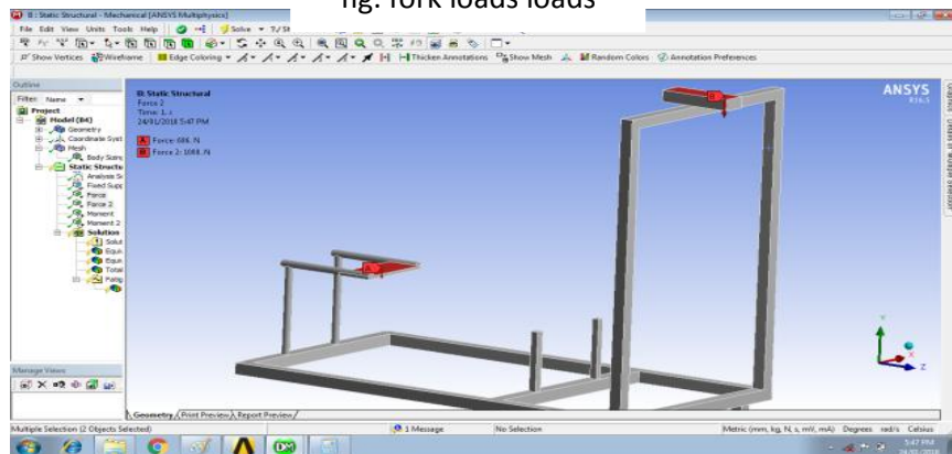
fig. fork lift forces
